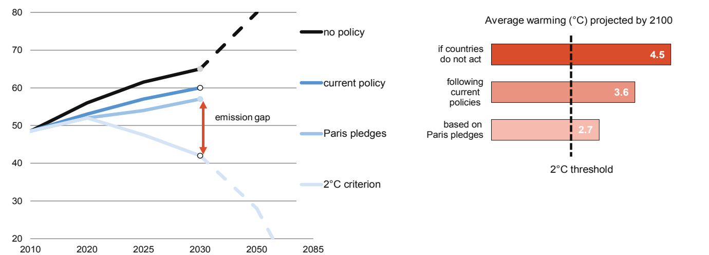
Figure 1.13 Global CO2 emission scenarios after Paris COP21 (GtCO2e*)
